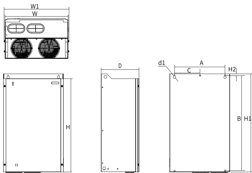
图 1-8 壁挂式安装尺寸图 (CP700-4T160-H~CP700-4T200-H、CP700-4T160-H-7.5~CP700-4T200-H-7.5)
